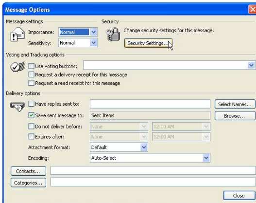
Fig. 4.2: Security Settings...
