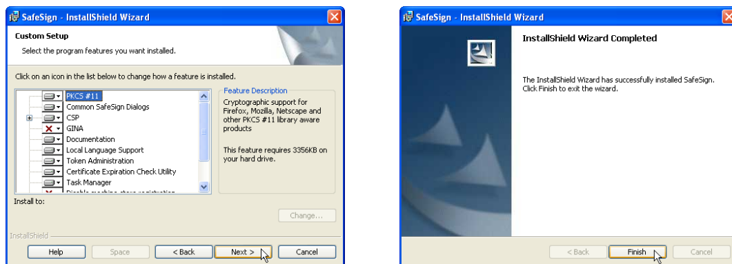
Fig. 2.3: SafeSign installation
